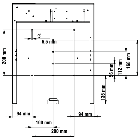
Variant Flex 21.5 lite
